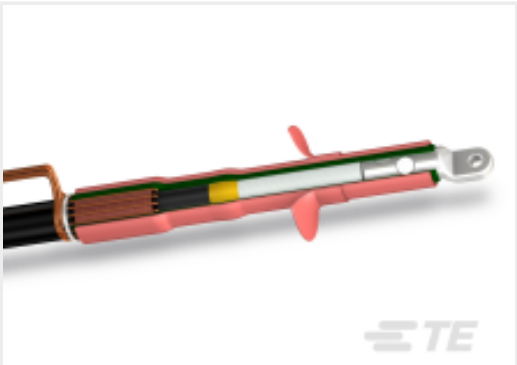
TE 产品编号D08155-064 POLT-42D/1XO-L12
