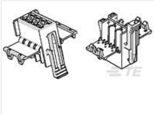
TE 产品编号1-929504-2 2X 3P JUN-POW-TIMGH
