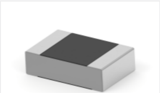
TE 产品编号1-2176238-0 CPF A 0805 30R 0.1% 25PPM 5K RL
