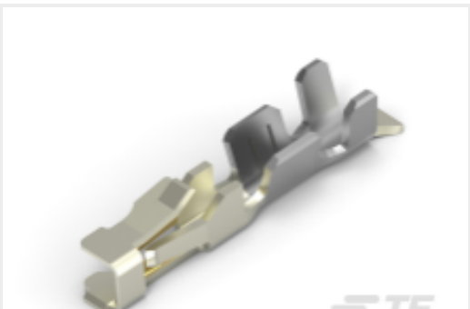
TE 产品编号3-2316113-4 2MM,REC,CNT,CRIMP,24-28AWG,0.1 UM,LP
