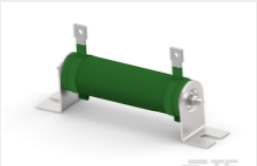
TE 产品编号5-1879441-0 TE 50W R47 5% Bracket
