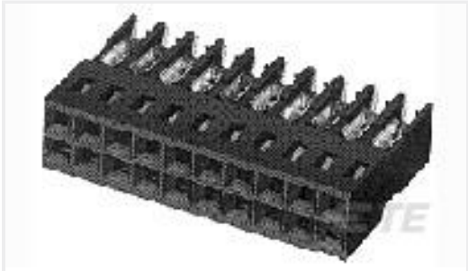
TE 产品编号5-102393-5 14 AMPMODU MT ASSY DR.100CL SN
