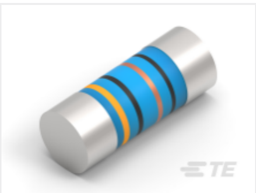
TE 产品编号2176315-4 MELF SMA_A 180R 0.1% 15PPM 0204 0.4W
