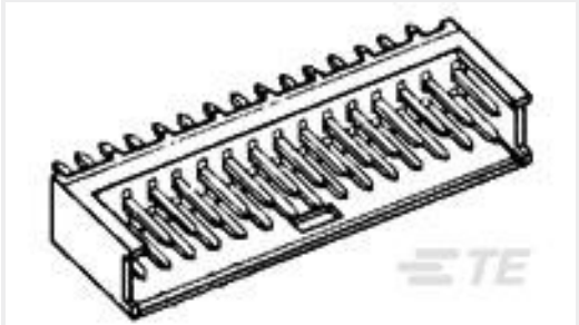
TE 产品编号280385-2 2X8P AMPMODU II SHRD HDR,ST,0.38 AU
