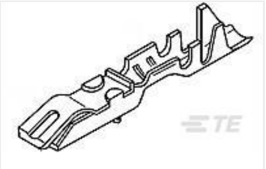
TE 产品编号867052-2 LOCKING CLIP CONT ASSY .025 SQ
