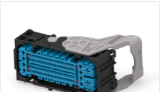
TE 产品编号2344715-8 90POS,HYBRID,REC HSG ASSY,SLD, COD A
