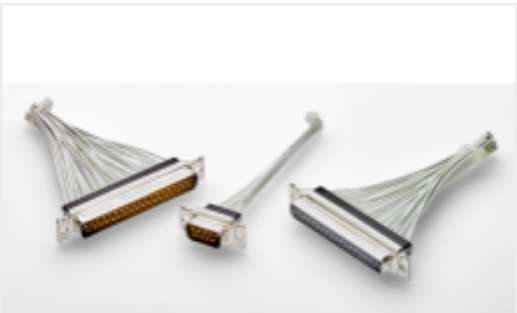
TE 产品编号2335893-2 AMPLIMITE SZ 2 RECPT 26 POS, ST STL SHEL
