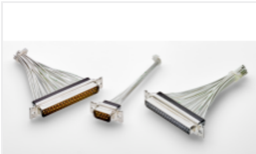
TE 产品编号2335893-5 AMPLIMITE SZ 5 RECPT 78 POS, ST STL SHEL
