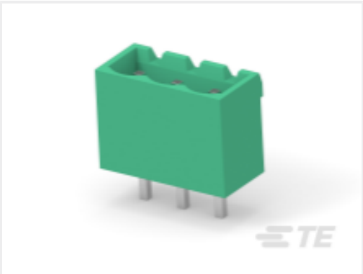
TE 产品编号2351885-3 3POS TB HDR 180 DEG, PITCH 5.0&TL 4.5mm
