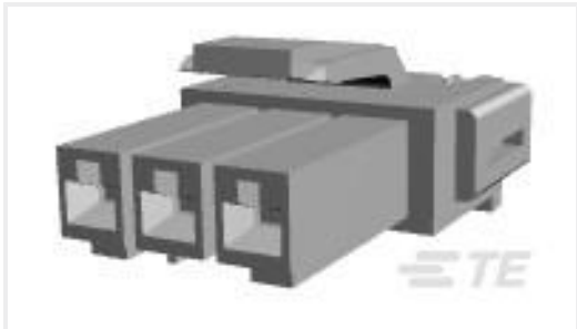
TE 产品编号177899-6 POWER DBL LOCK PLUG HSG 3P
