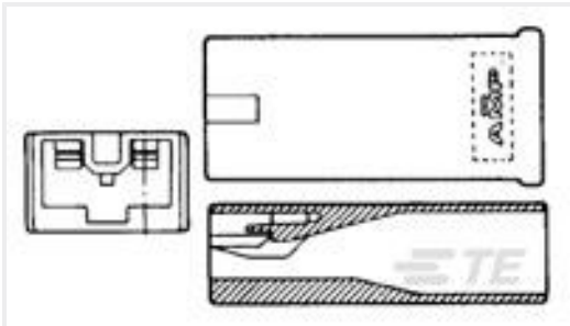
TE 产品编号179970-9 PL EXII 250 REC HSG 1P NYLON BLACK
