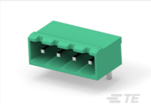
TE 产品编号2350513-4 4POS TB HDR 90 DEG, PITCH 5.0 & TL 4.5mm
