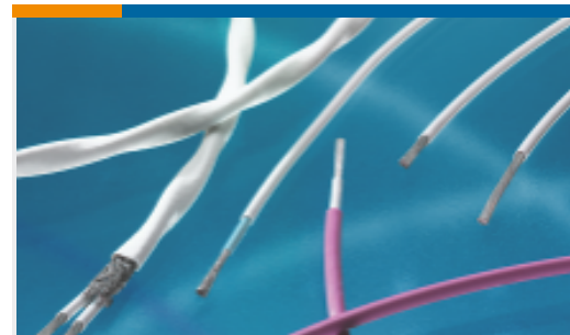
TE 产品编号316034-006 General Purpose 2 Core Cable: Tin Coated Copper, 22 AWG
