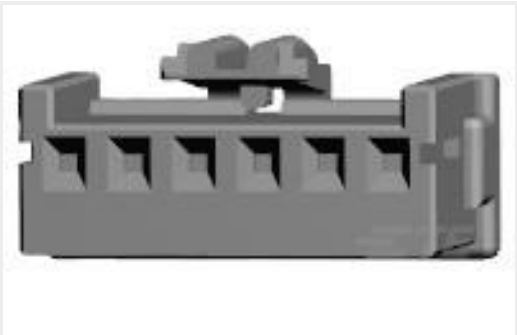
TE 产品编号917690-1 2.5 SIGNAL D/LOCK PLUG HSG 6P
