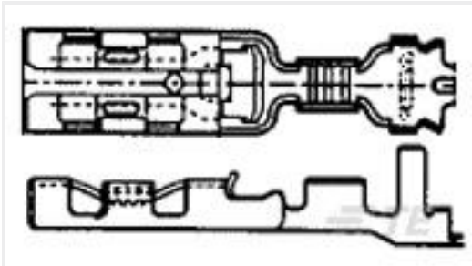
TE 产品编号353250-2 110 PL EX REC. 20-16AWG PTPHBZ
