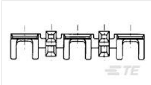
TE 产品编号353256-1 110 HSG. PL EX REC. 7.6mm 3P NAT
