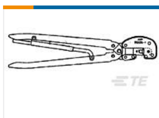
TE 产品编号234171-1 HHHT DYNAMIC D-5 M 12-10 ASSY
