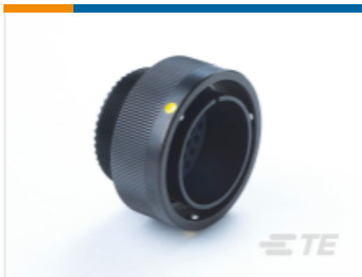
TE 产品编号Y5015-000000100017 FREE PIN CONNECTOR
