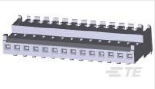
TE 产品编号4-644540-4 14P MTA100 CONN ASSY F/T POL
