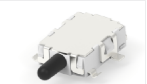
TE 产品编号2331391-1 DET SW5.7X4.0X2.0 GW HORZ. NC AG RL
