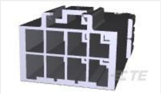
TE 产品编号179467-6 AMP POWER DBL LOCK CAP HSG 8P
