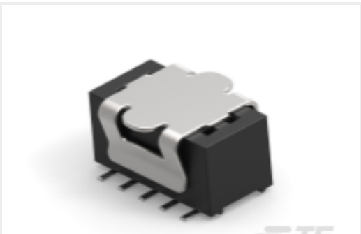
TE 产品编号2267465-5 SCL 1.0 RCPT DR VT 010 SMT G1 TBK
