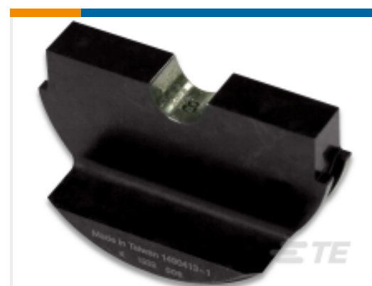
TE 产品编号1490413-1 HYP10 SOLIS 8AWG NEST
