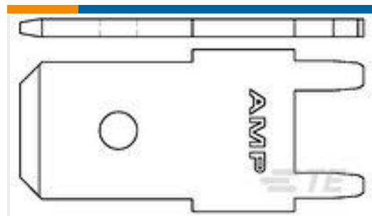
TE 产品编号1-1217056-0 250 FASTON,PCB TAB,TPBR
