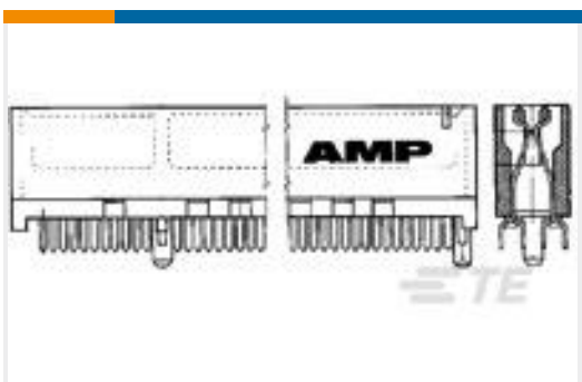
TE 产品编号5650181-3 STANDARD EDGE .050 SERIES 23 DUAL ASSY
