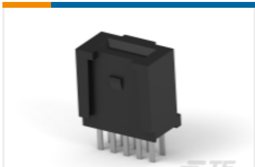
TE 产品编号1766966-1 CONNECTOR, SOCKET, COMPLIANT, FLATPAQ
