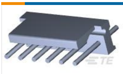
TE 产品编号3-644760-6 06P MTA156 HDR ASSY FL ST LF
