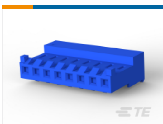
TE 产品编号 3-643821-8 08P MTA156 CONN ASSY 26AWG LF
