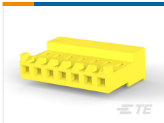
TE 产品编号 3-643818-7 07P MTA156 CONN ASSY 20AWG YEL
