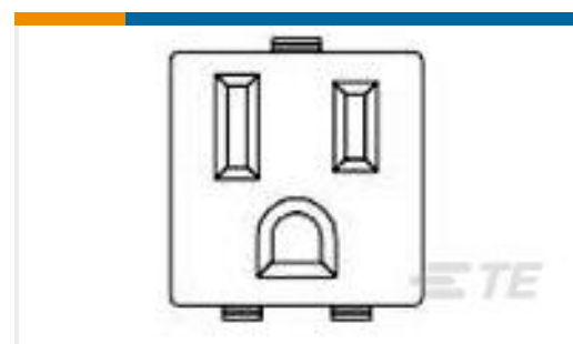
TE 产品编号3-213598-2 CNV OUTLET PCBOARD MNT,BLK LF
