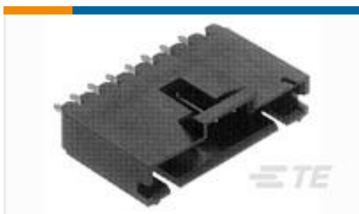
TE 产品编号5-103639-5 06 MTE HDR SRST LATCH .100CL
