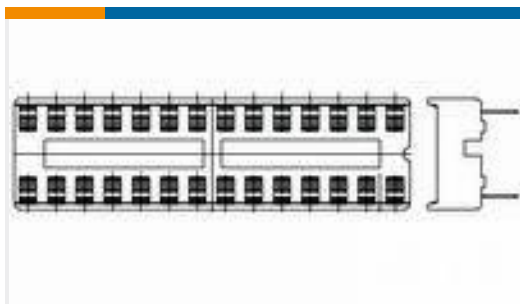
TE 产品编号1-2199298-4 16P,DIP SKT,300 CL,LDR,PB FREE
