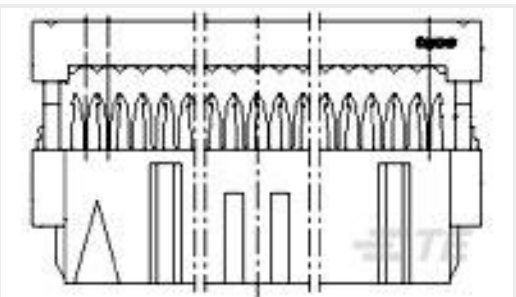
TE 产品编号1-215915-0 AMP-LATCH 15.2 HIGH TAPE
