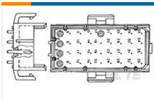
TE 产品编号640506-2 36P MR HDR ASSY V0
