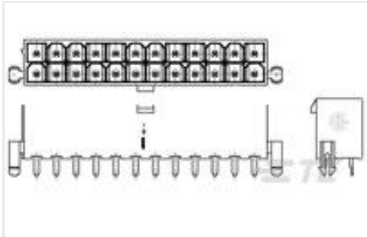
TE 产品编号1-2029265-6 16P VAL-U-LOK VRTHDR W/PGS GW
