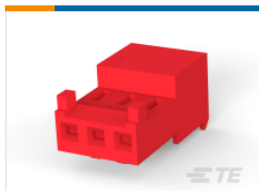
TE 产品编号4-643814-2 Nylon Tin Plated Receptacle: 2.54 mm, with Mating Alignment, MTA 100
