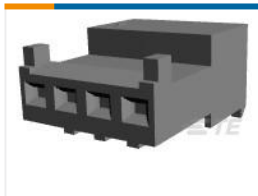
TE 产品编号3-643814-4 04P MTA100 CONN ASSY POL RIB
