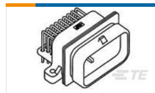
TE 产品编号6437288-3 SUPER SEAL 60POS CAP ASSY H AU
