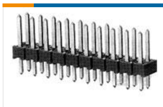
TE 产品编号5-146261-6 12 MODII HDR DRST B/A .100CL LF
