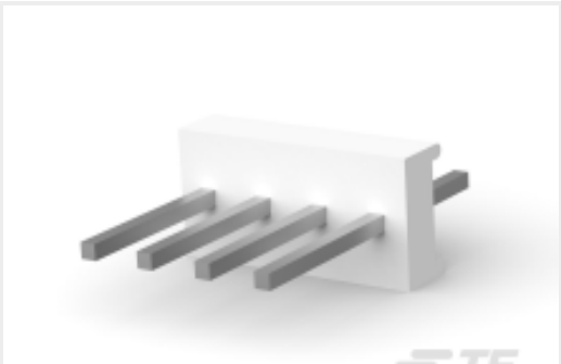
TE 产品编号CAT-104MTA-PVUNH PCB Header: Polyester, Vertical, Unshrouded, No Mating Alignment
