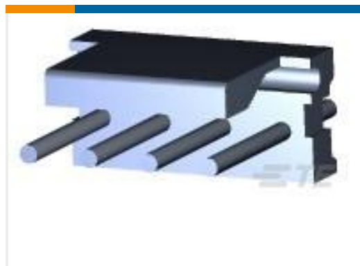
TE 产品编号3-641120-4 04P MTA156 HDR ASSY FL/ST LF
