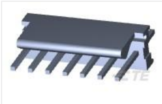
TE 产品编号3-641215-7 07P MTA100 HDR ASSY FL/ST 30AU
