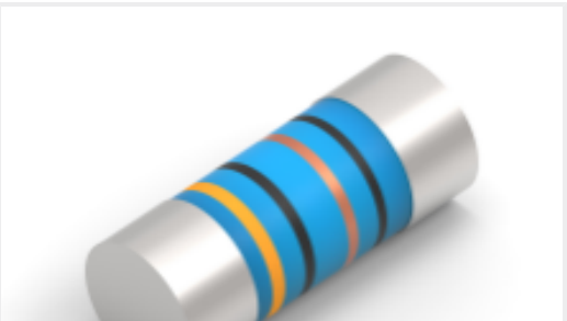
TE 产品编号8-2176315-3 MELF SMA-A 47R 1% 50PPM 0204 0.4 W
