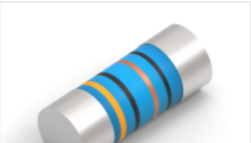
TE 产品编号7-2176315-9 MELF SMA-A 22R 1% 50PPM 0204 0.4 W
