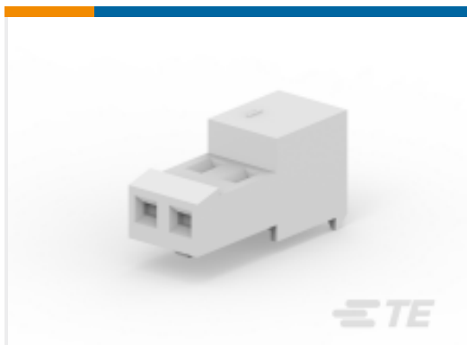
TE 产品编号3-641537-2 MTA Receptacle: Nylon, Tin Plated, 2.54 mm
