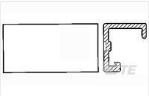
TE 产品编号640550-8 08P MTA100 COVER
