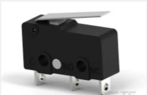
TE 产品编号2351451-1 SMINSA SW HLV1.47N 5A/3A AC 3A DC SP
