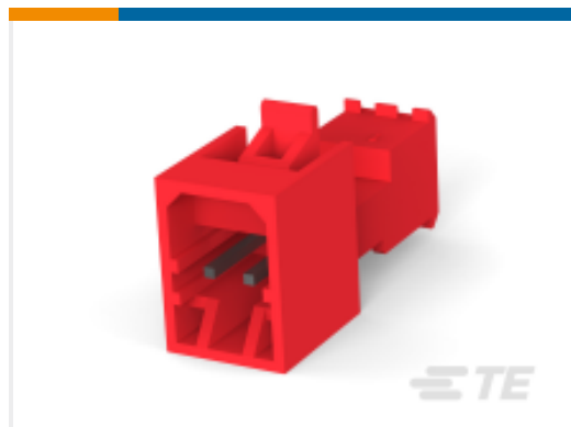
TE 产品编号3-647000-3 MTA Plug: Nylon, Tin Plated, 2.54 mm, with Mating Alignment
