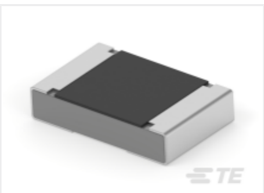
TE 产品编号9-2176483-4 RA73F 2A 5K11 0.1% 5K RL
