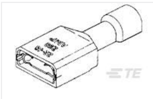
TE 产品编号3-520150-2 ULTRA-FAST 187 ASY REC 16-14 AWG TPBR
