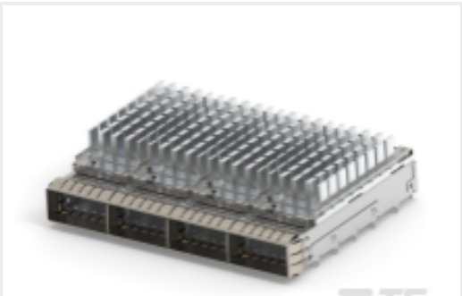
TE 产品编号2170790-7 CAGE ASSY, 1X4, QSFP28, SPRING, HS
