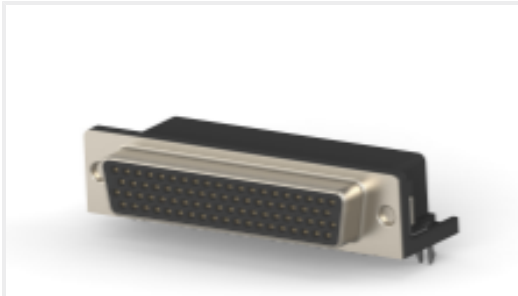
TE 产品编号2311772-1 AMPL REC, HD22, R/A, 78P, THREADED
